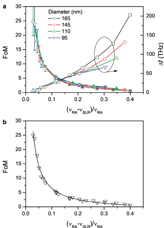
Figure 4. Measured FoM for different gold nanoparticle arrays and fit of the experimental data. (a) Experimental FoM ( \partial\lambda/\partial n )/ \Delta\lambda and the full width at half-maximum \Delta f of surface lattice resonances as a function of the parameter \delta = (\nu_{RA} - \nu_{SLR})/\nu_{RA} for particle arrays with diameters 95, 110, 145, and 165 nm, height 50 nm, and lattice constant a = 300, 350, 400, 450, 500, 550, and 600 nm. (b) The solid line is a fit to the experimental data (symbols) indicating a reciprocal scaling of the FoM with \delta .
